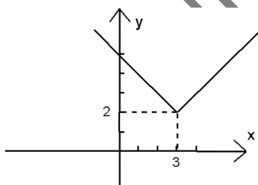
graph of f(x) = |x - 3| + 2
